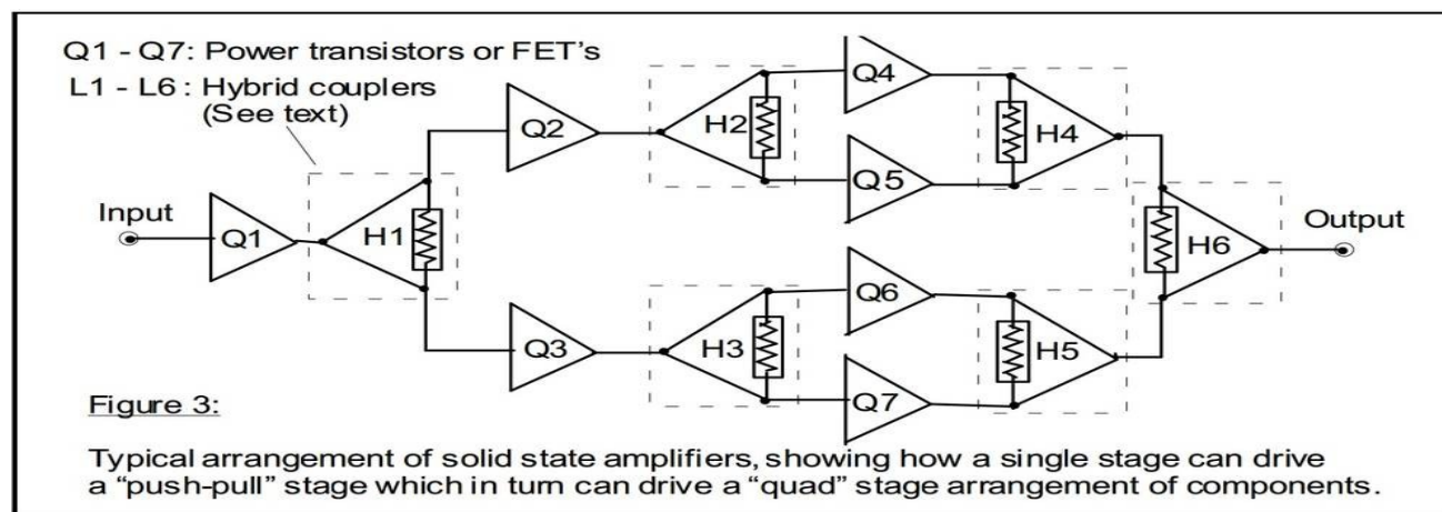
Figure 3 shows, in block diagram form, the typical arrangement of components in solid state amplifiers. In these circuits, the active devices are usually operated in a Class "B" mode, drawing a very small amounts of current until excited by a driving
